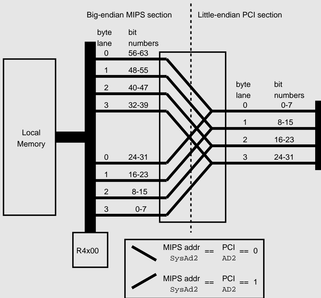
Figure 11.8: Writing a big-endian CPU to a little-endian bus
