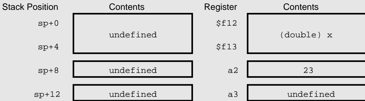
Figure 10.2: Argument structure, A floating-point arguments
