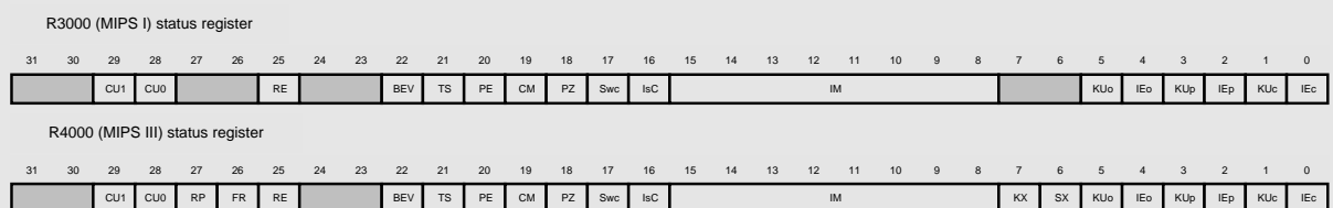
Figure 3.2: Fields in status register SR
