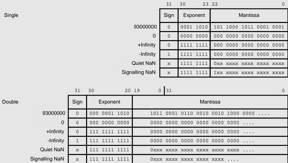
Figure 7.1: Floating-point data format
