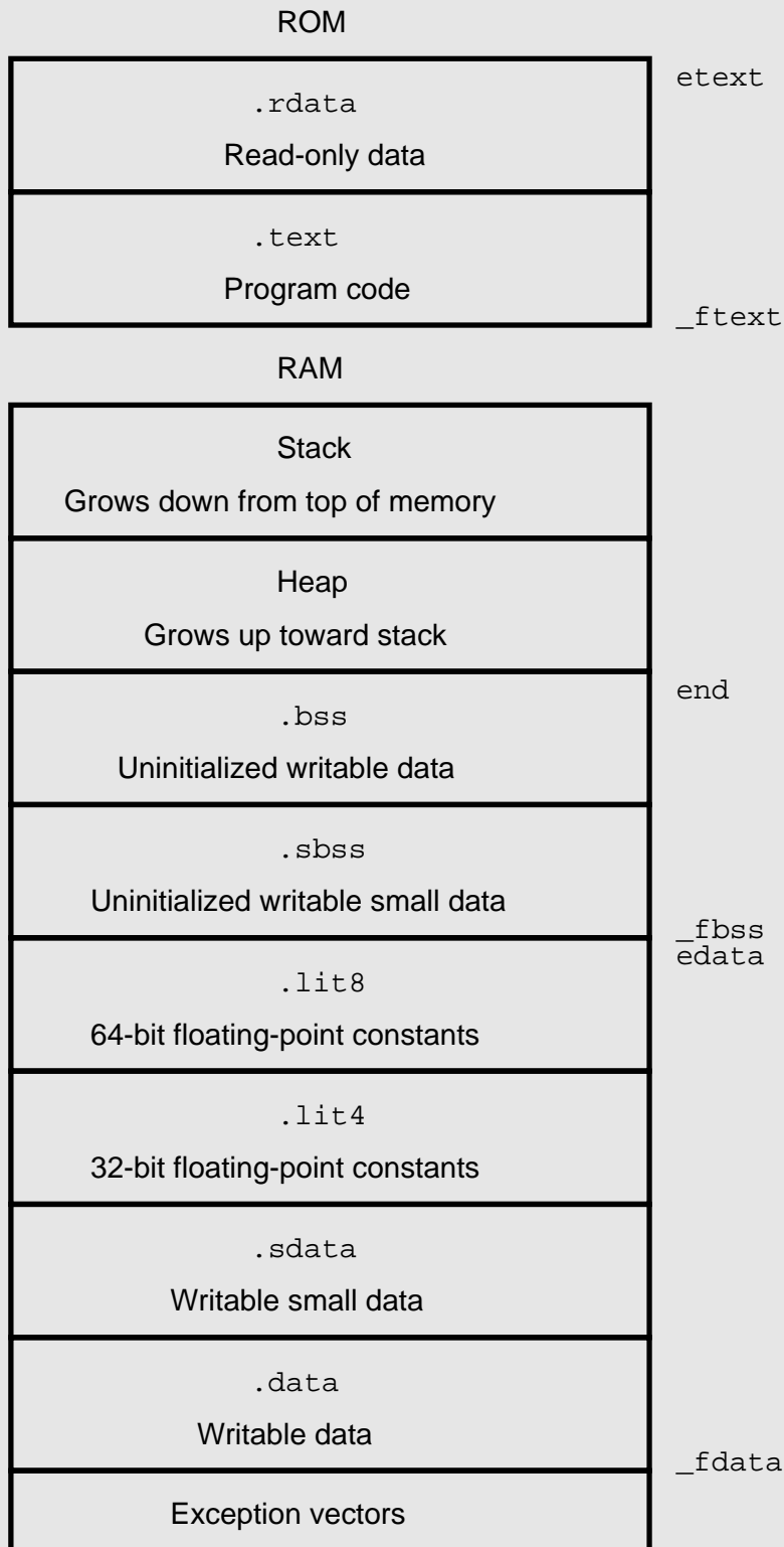
Figure 9.1: ROMable program’s object code segments and typical memory layout
