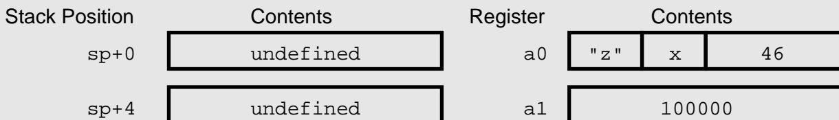
Figure 10.3: Arguments when passing a structure type
