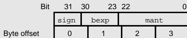
Figure 11.6: Bitfield from the big-endian viewpoint
